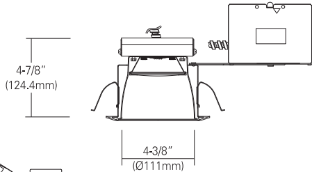
Ceiling Cut-out : 5"
