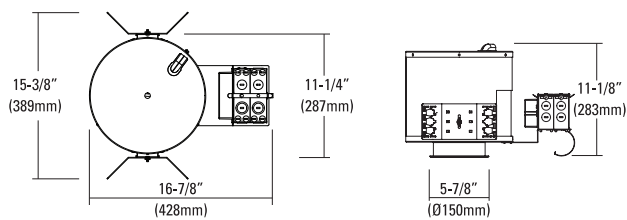
Ceiling Cut-out : Ø5-1/2" (Ø140mm)
